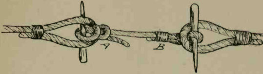
FIG. 100.—Belaying-pin splice.
